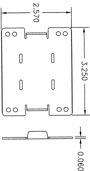
8 3-PIECE CLIP BASE (33 KSI STEEL)
